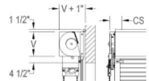
CHAIN HOIST MODEL: HWFC
