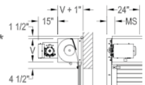
MOTOR OPERATOR* MODEL: HWFM
