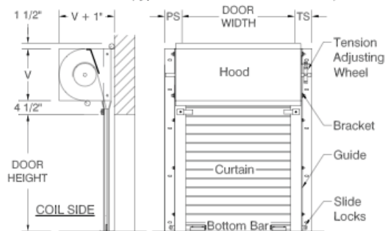
PUSH-UP MODEL: HWFP
