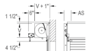
AWNING CRANK* MODEL: HWFA (To 16' wide, 10' high 150 sq. ft.)
